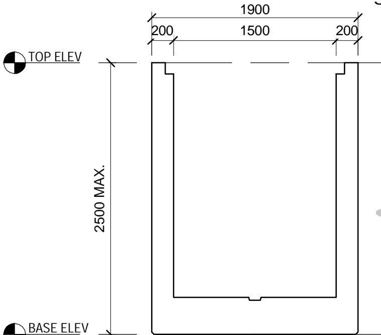
FRONT ELEVATION
