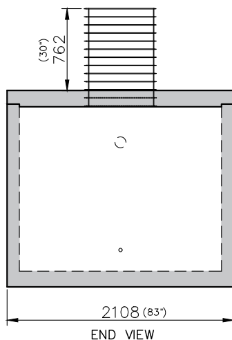
END VIEW
