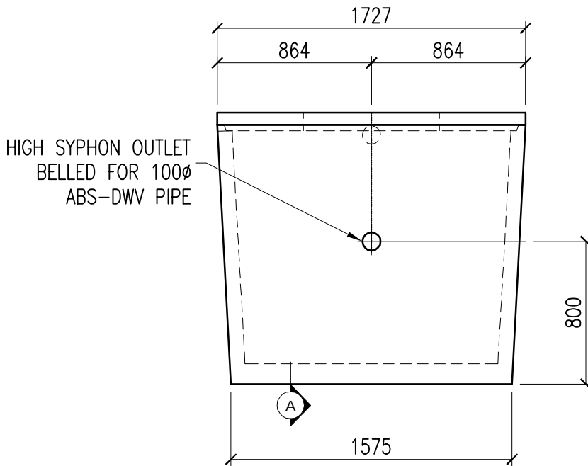
END VIEW
