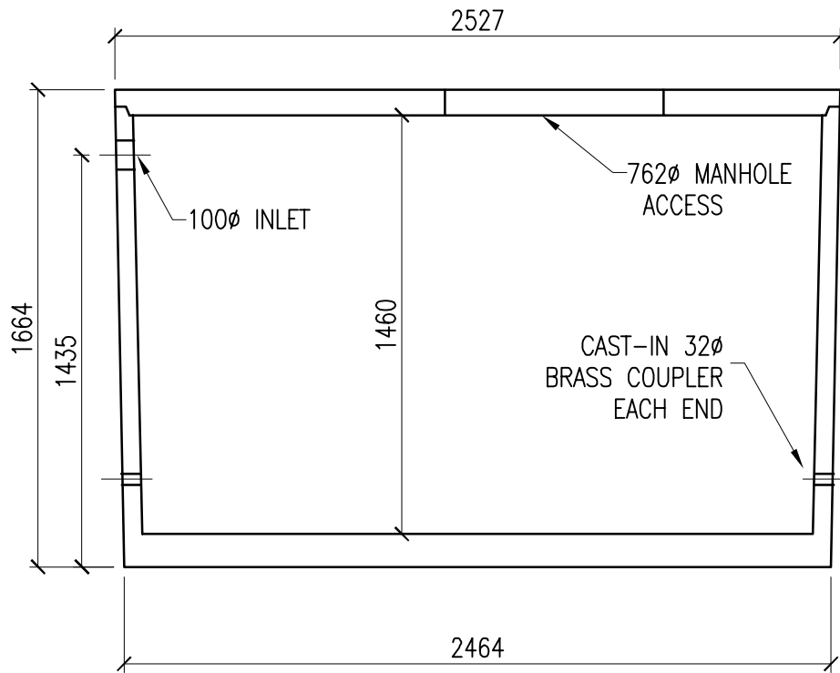
SECTION A
