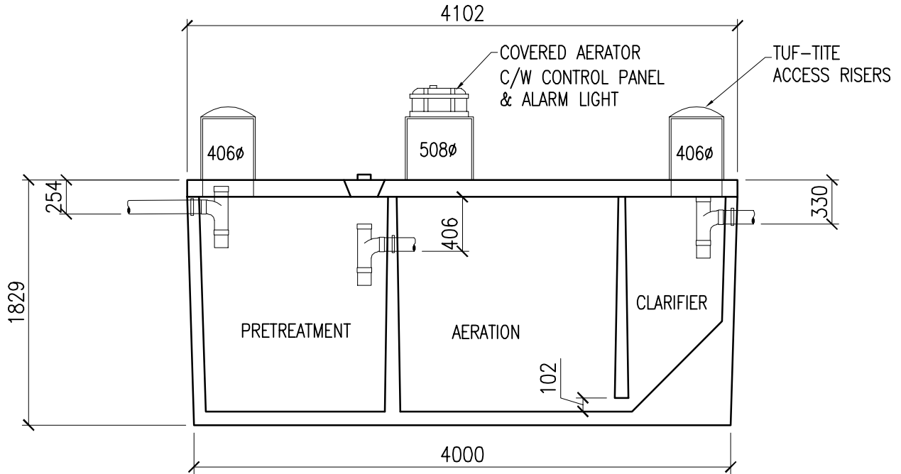
SECTION A
