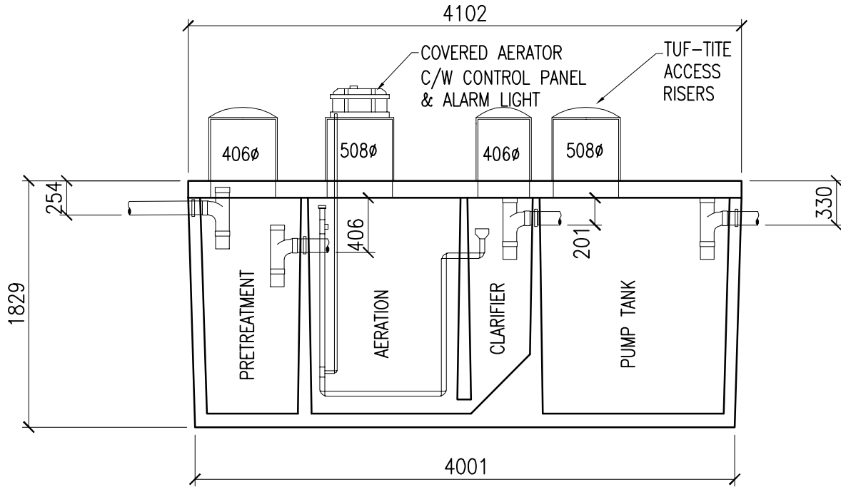
SECTION A
