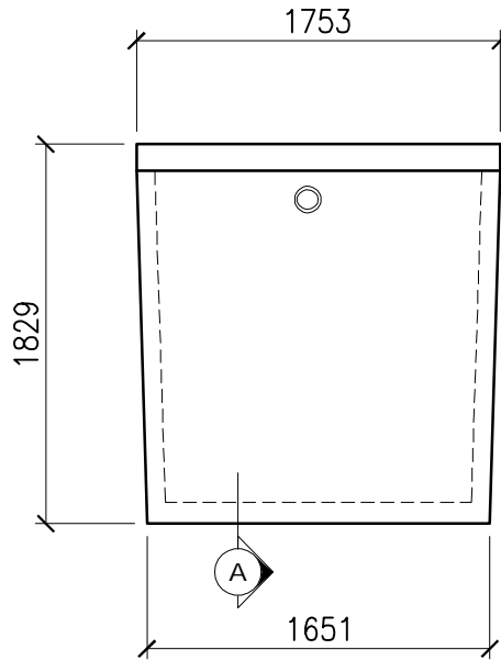
END VIEW
