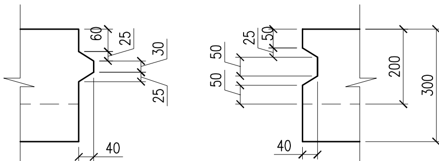
KEYWAY DETAIL
