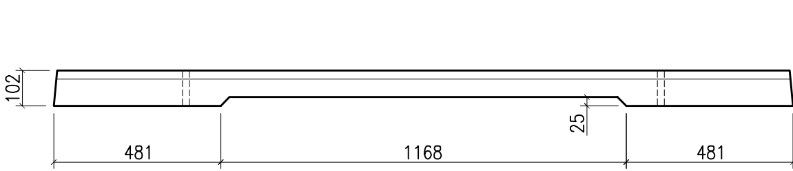
SIDE VIEW A
